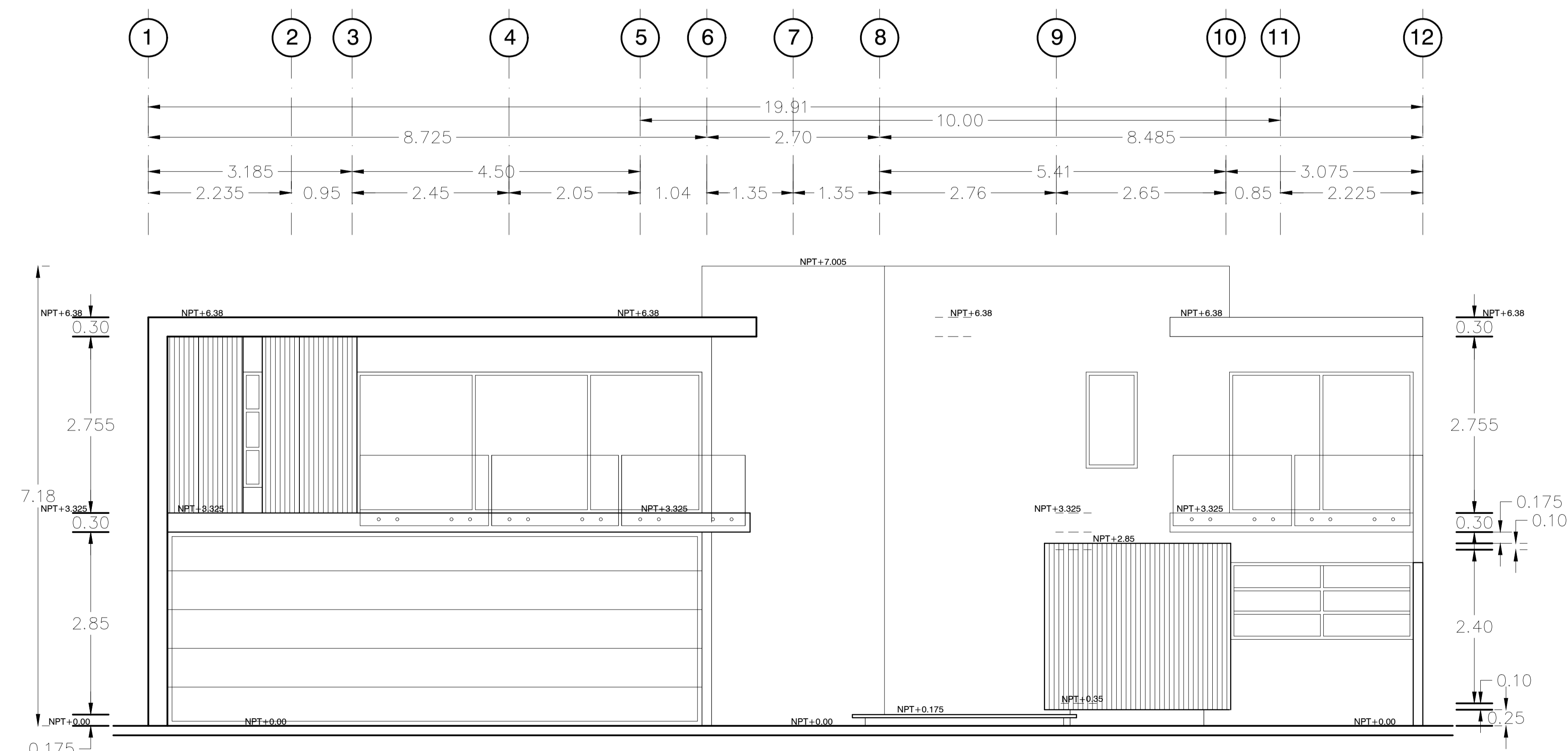
FACHADA PRINCIPAL
